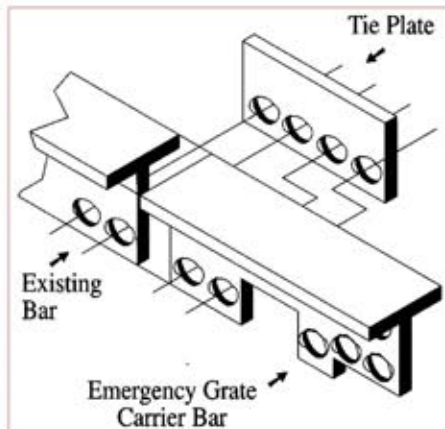
Indeck Keystone Energy Emergency Grate Carrier Bar
